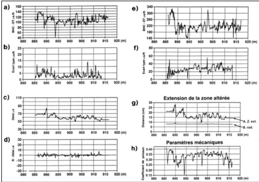
Figure 3.10 Example of acoustic logs in a sandstone reservoir (from Coppens and Mari, 1995). Monopole tool: (P wave): a) Slowness; (b) Standard deviation of slowness; (c) Delay; (d) Residual delay. Dipole tool (bending wave # S wave): e) Slowness; (f) Standard deviation of slowness; (g) Extension of the weathering zone (P wave); (h) Poisson's ratio.
