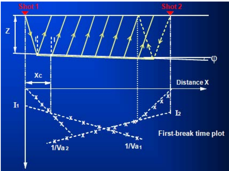
Figure 2.1 Intercept-time method.
