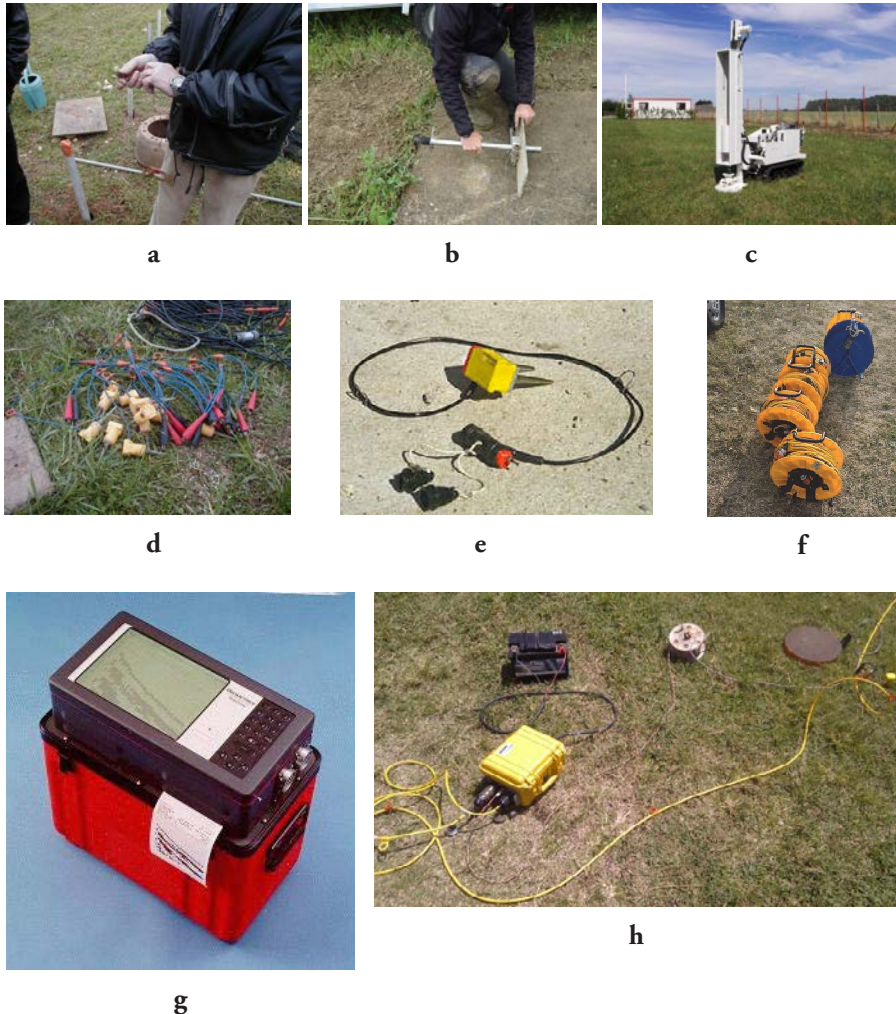
Figure 2.6 Field equipment. Source: explosive, gun, weight drop (a, b, c: Apec document); sensors: vertical and horizontal geophones (d, e: IFPEN document), cables (f: IFPEN document); recorders: Geometrics Strataview (g: IFPEN document), Geometrics geode (h: GEO2X document).
